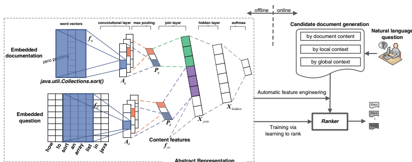
Figure 2: The architecture of QDLinker.
