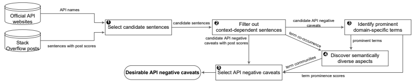
Figure 3: Overview of the DISCA framework.
